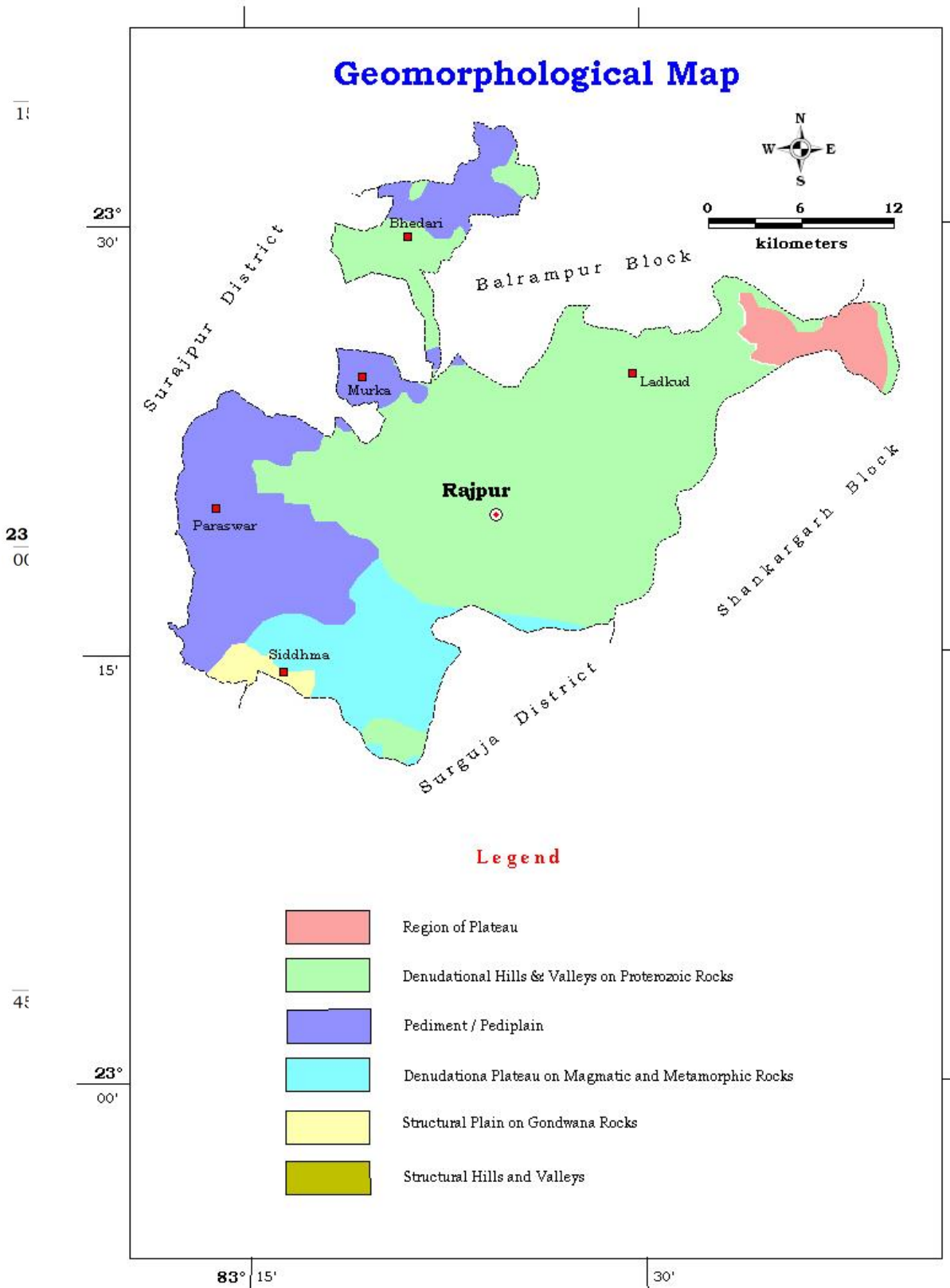
Figure 2 Geomorphology Map of Rajpur Block
